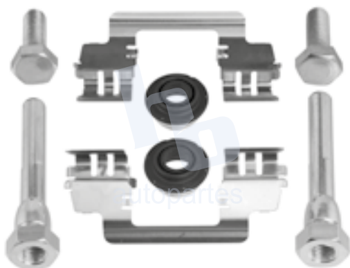
KIT DE CALIPER RUEDA DELANTERA CHRYSLER 300 (05-18), CHALLENGER (09-17), DODGE CHARGER (06-22) 7962 D1056, 7965 D1058.
