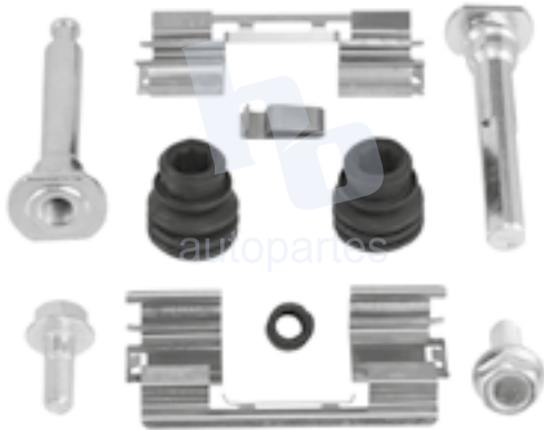
KIT DE CALIPER RUEDA TRASERA CHEVROLET COLORADO (15-19), GMC CANYON (15-19) 9041 D1806.
