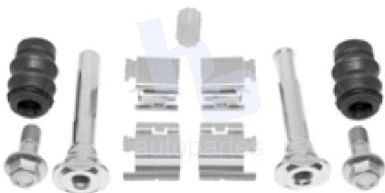
KIT DE CALIPER RUEDA TRASERA FORD TRANSIT (10-12), MERCEDES BENZ SPRINTER (07-19), NISSAN CABSTAR (08-16), VOLKSWAGEN CRAFTER 3.5 TONS (08-12) 8432 D1318.
