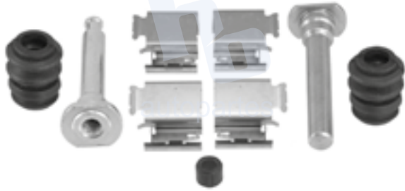
KIT DE CALIPER RUEDA DELANTERA FORD TRANSIT 150, TRANSIT 250, TRANSIT 350 (15-18) 9004 D1774
