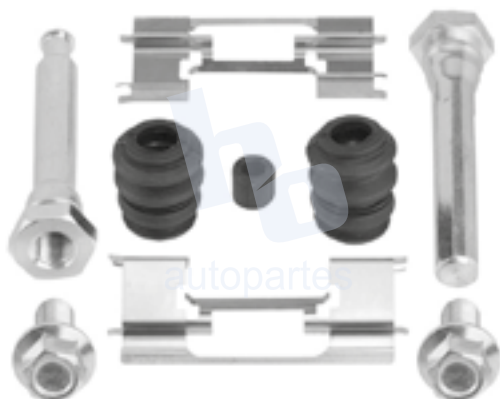
KIT DE CALIPER RUEDA DELANTERA HONDA ACCORD EX (13-20), ACCORD EXL (13-20), ACCORD HYBRID (13-18), HRV (16-18) 8883 D1654.
