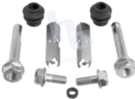
KIT DE CALIPER RUEDA TRASERA AM GENERAL HUMMER H3 (06-10), 8226 D1120.
