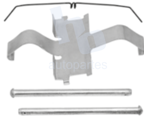
KIT DE CALIPER RUEDA DELANTERA TOYOTA HILUX (05-17) 8776 D1567, JAC FRISON (19-22) 7877 D976.
