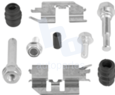
KIT DE CALIPER RUEDA TRASERA SUBARU FORESTER 2.5L (14-15), IMPREZA (08-15), LEGACY (05-15), OUTBACK (05-15), SUBARU TRIBECA (08-14) 8218 D1114.
