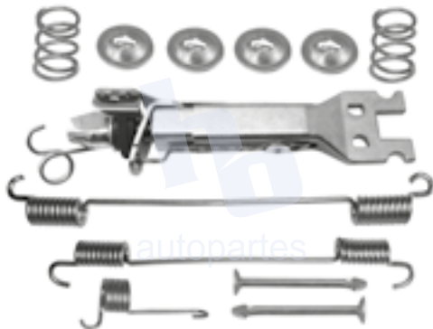
KIT PARA FRENO DE TAMBOR RUEDA TRASERA FIAT PALIO (04-11), STEPWAY (10-11) 1601 887, RENAULT KANGOO (07-09), KANGOO EXPRESS (04-19) 1Y28Z FT038.
