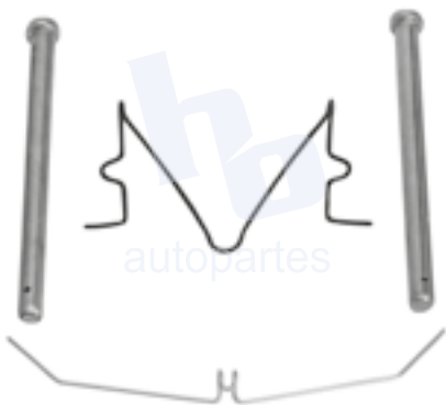
KIT DE CALIPER RUEDA DELANTERA TOYOTA 4RUNNER (84-89), PICK UP (89-95) 7549 D436.
